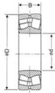
With oil groove and oil holes (W33)
