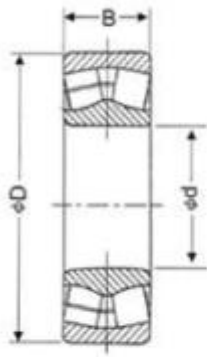
Cylindrical bore
